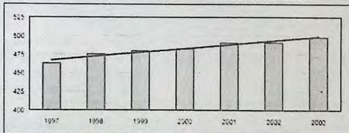
KWH (CONSUMPTION) / KVA (CAPACITY) Load Shape in KWHs/KVA : Year-To-Date
