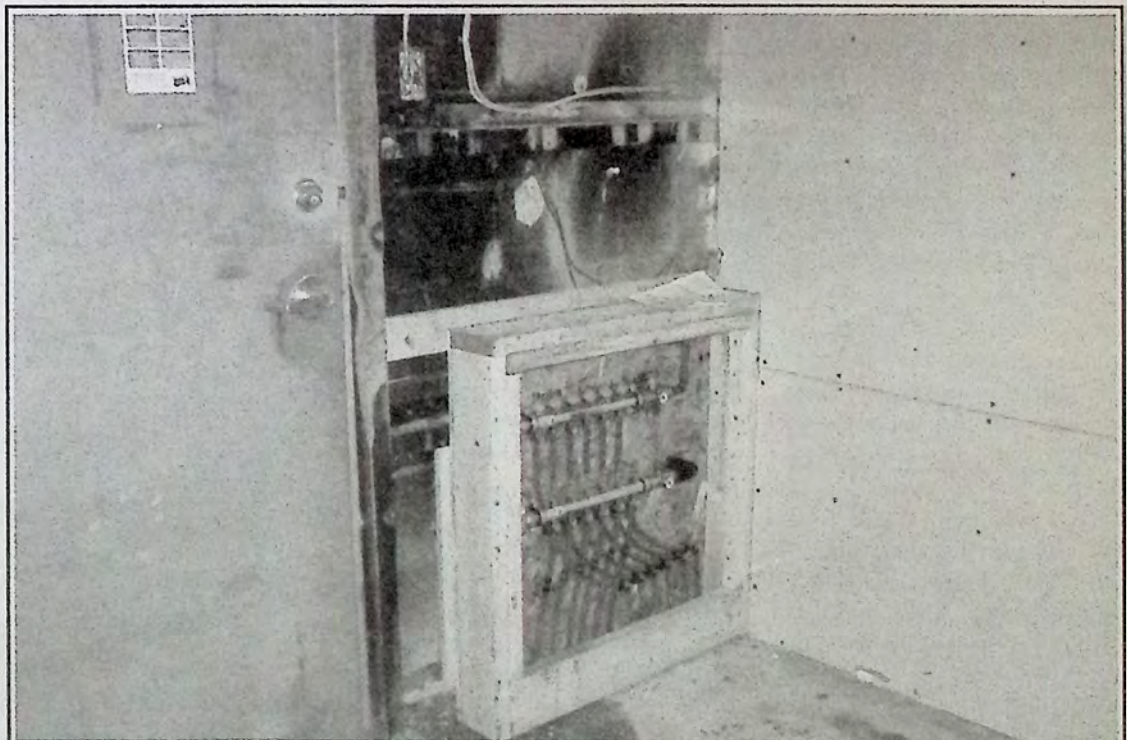
The radiant heat control panel was installed November 18th. Evidence of the fire that destroyed the building can still be seen above the panel. The system pumps warm water through tubing in the floor. *
