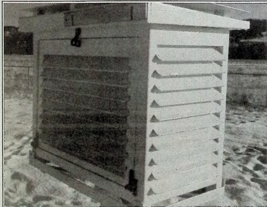
A Stevenson Screen is an enclosure to shield meteorological instruments against precipitation and direct heat radiation. Photo: Brenda Engel
