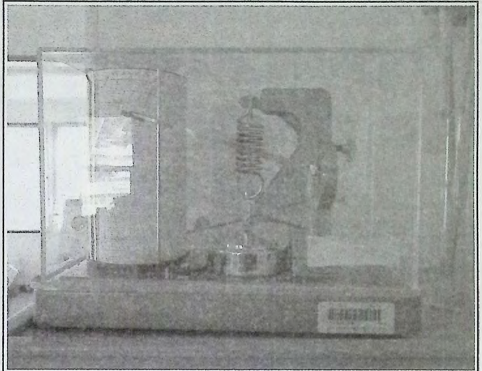
The Barograph produces a paper or foil chart called a barogram which records barometric pressure over a specific period of time. Photo: Brenda Engel
