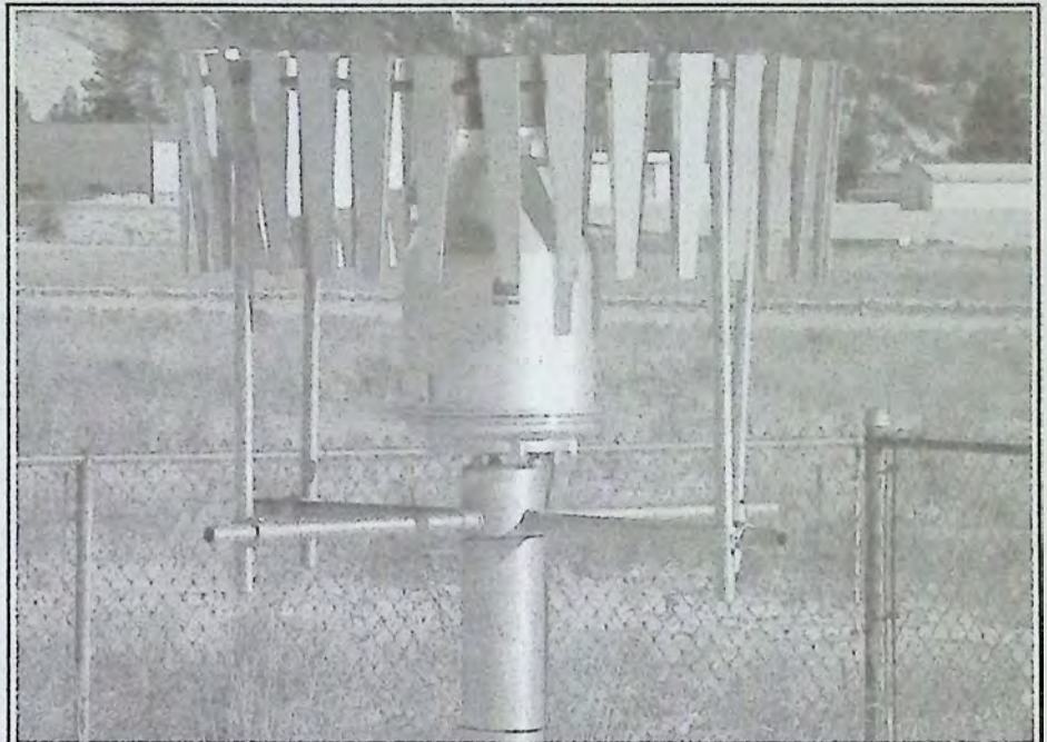
The Geonor is designed for year round measurements of accumulated precipitation (solid or liquid) as well as precipitation intensity. The amount of precipitation is measured by it's unique vibrating wire weighing transducer. This information is automatically fed to Environment Canada. Photo: Brenda Engel
