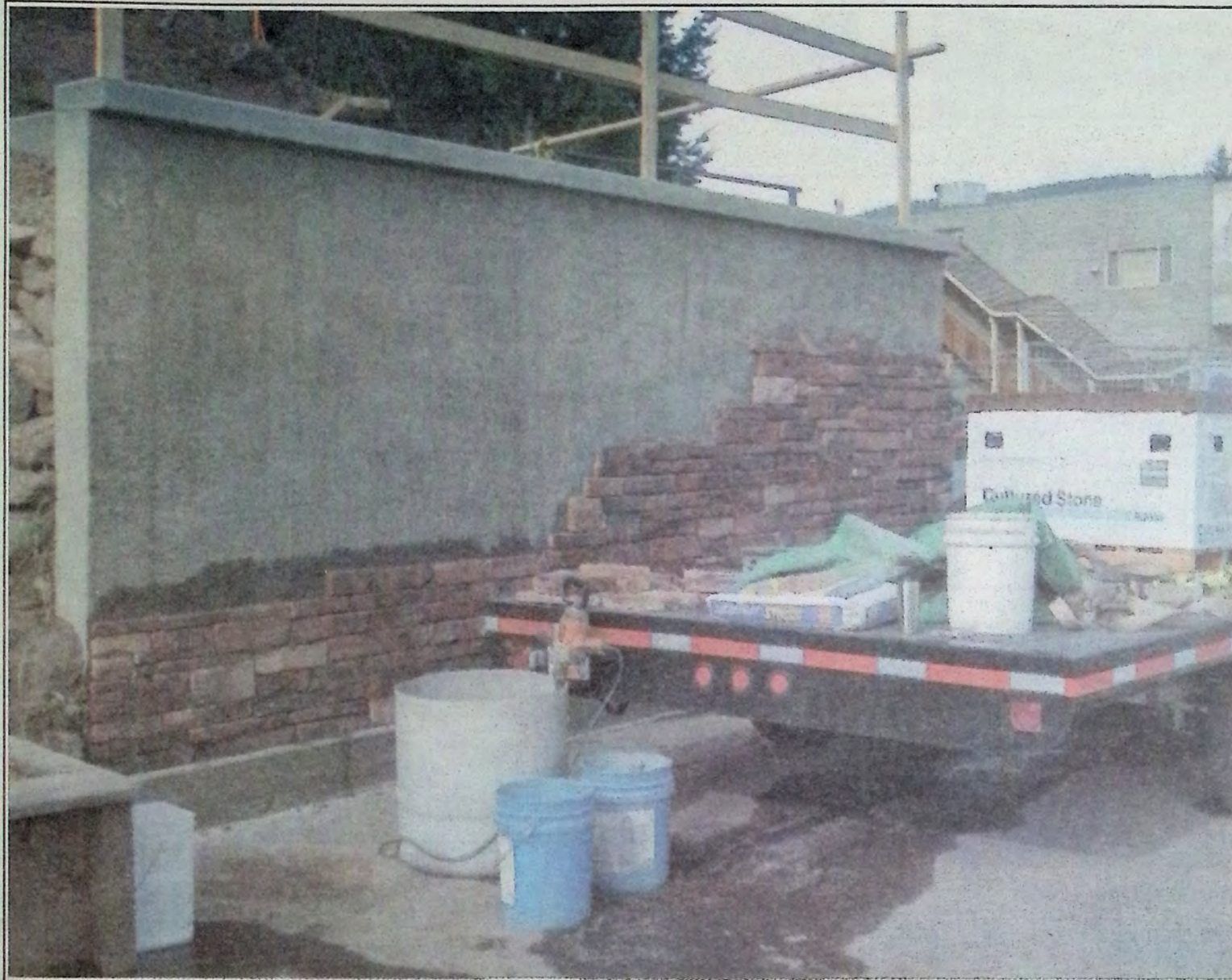
Cultured stones were applied to the retaining wall at the bottom of the zigzag project September 5th. Photo: Brenda Engel
