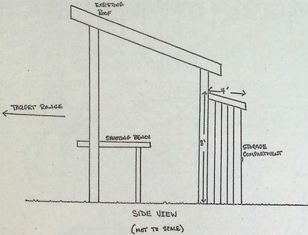
Sketch shows a side view of the plan to build a storage space at the gun range. Sketch: Princeton Fish & Game Club
