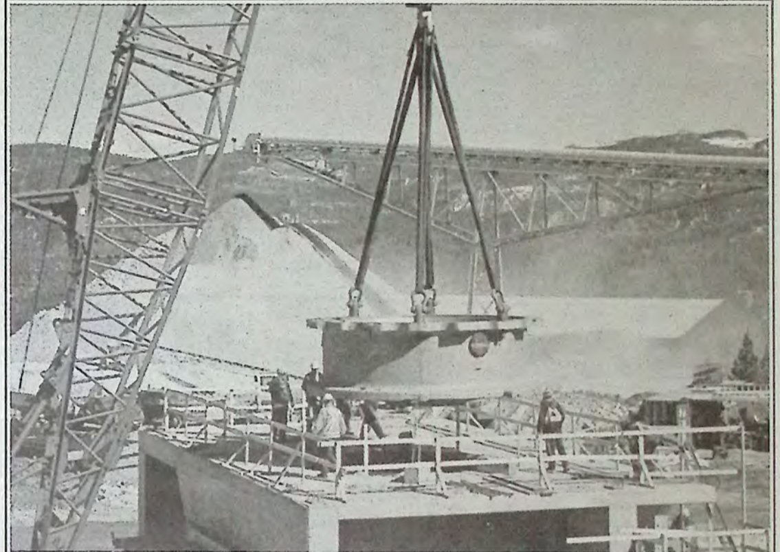
Workers at Copper Mountain Mine assist the lowering of the lower mainframe of the Raptor 2000 secondary crusher. The unit will take a number of weeks to fully assemble before becoming operational. Photo: Copper Mountain Mine
