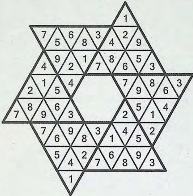
Hoshi Sudoku Solution - Medium
