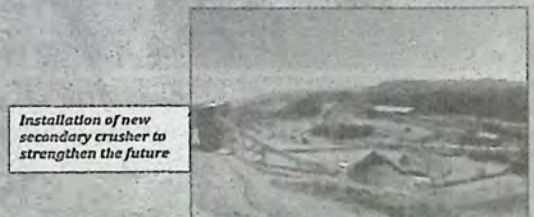
Ore which enters the primary crusher will be further reduced in size by the secondary crusher before it is sent into the SAG mill for grinding.
